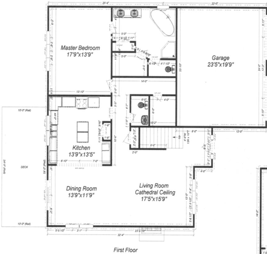
First Floor
